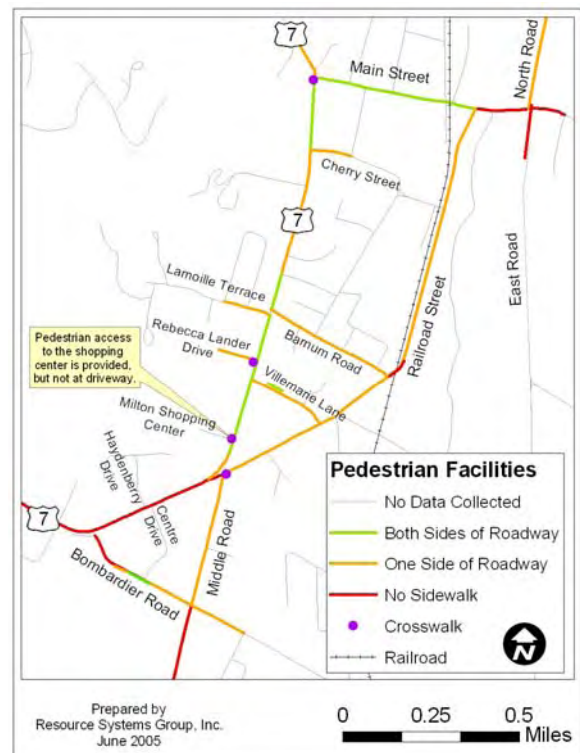
Figure 9: Milton Sidewalk System with Crosswalks
