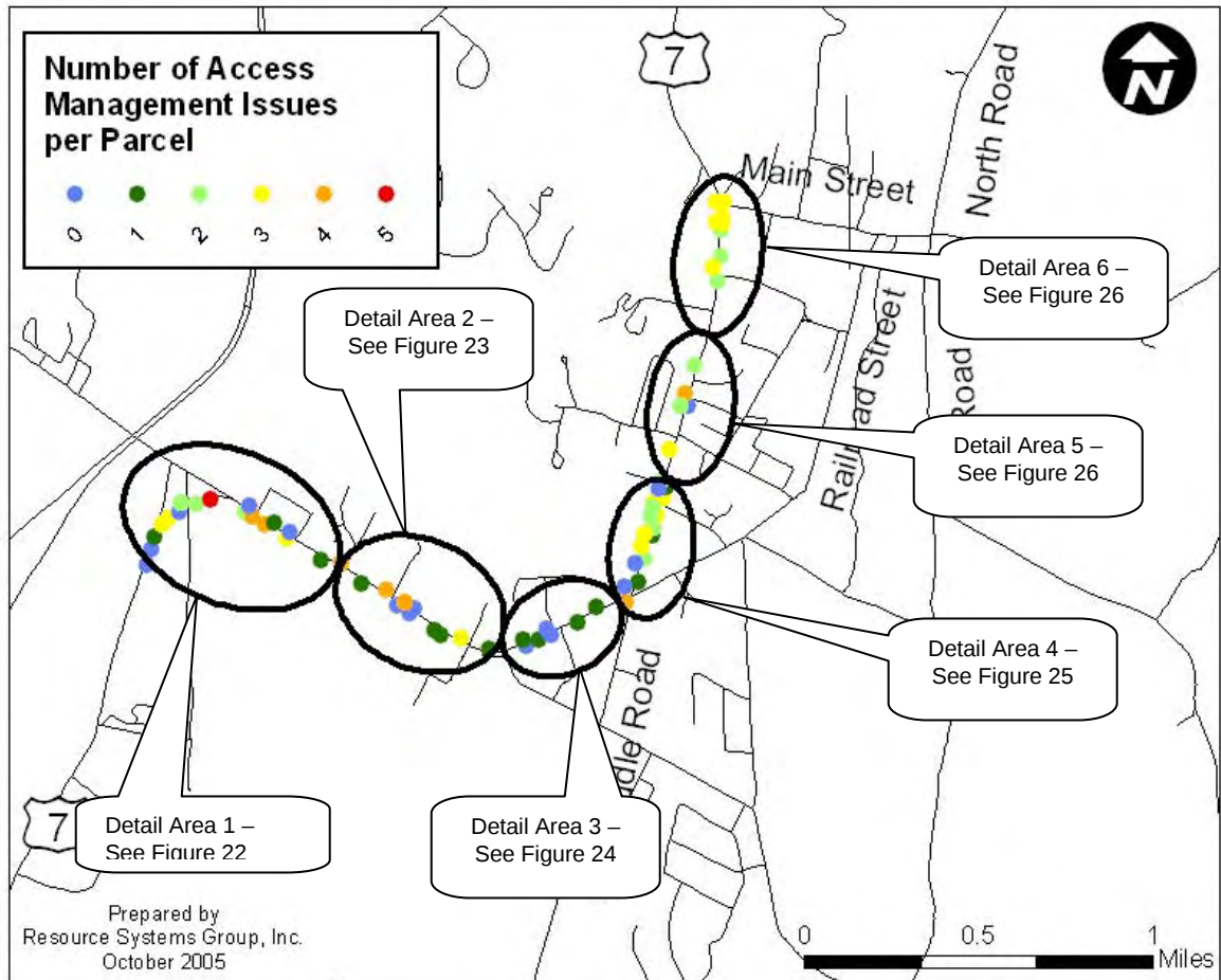
Figure 21: Access Management Issues along US 7
