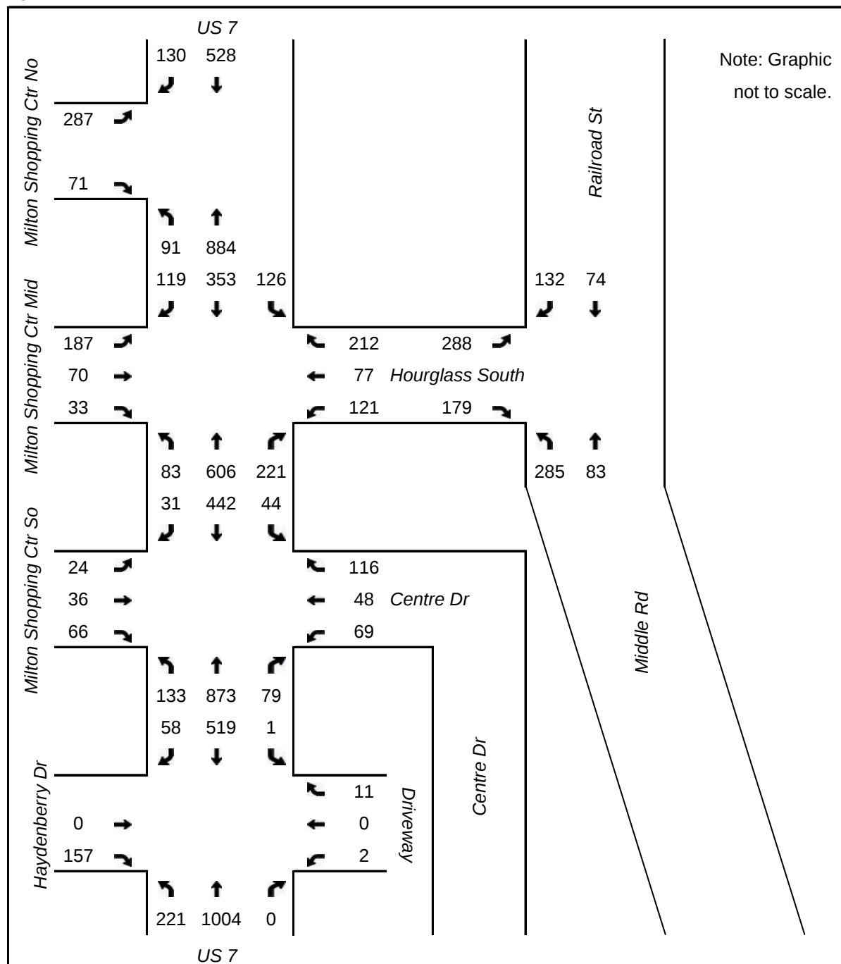
Figure 7: 2012 PM Peak Hour Scenario Volumes
